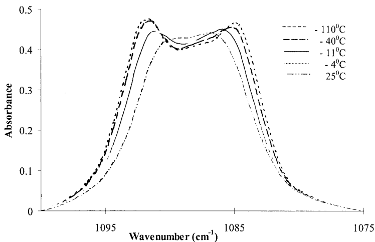
Figure 11. Reduction in \text{CD}_2 bending splitting in alkane with deuterated end groups with annealing.
